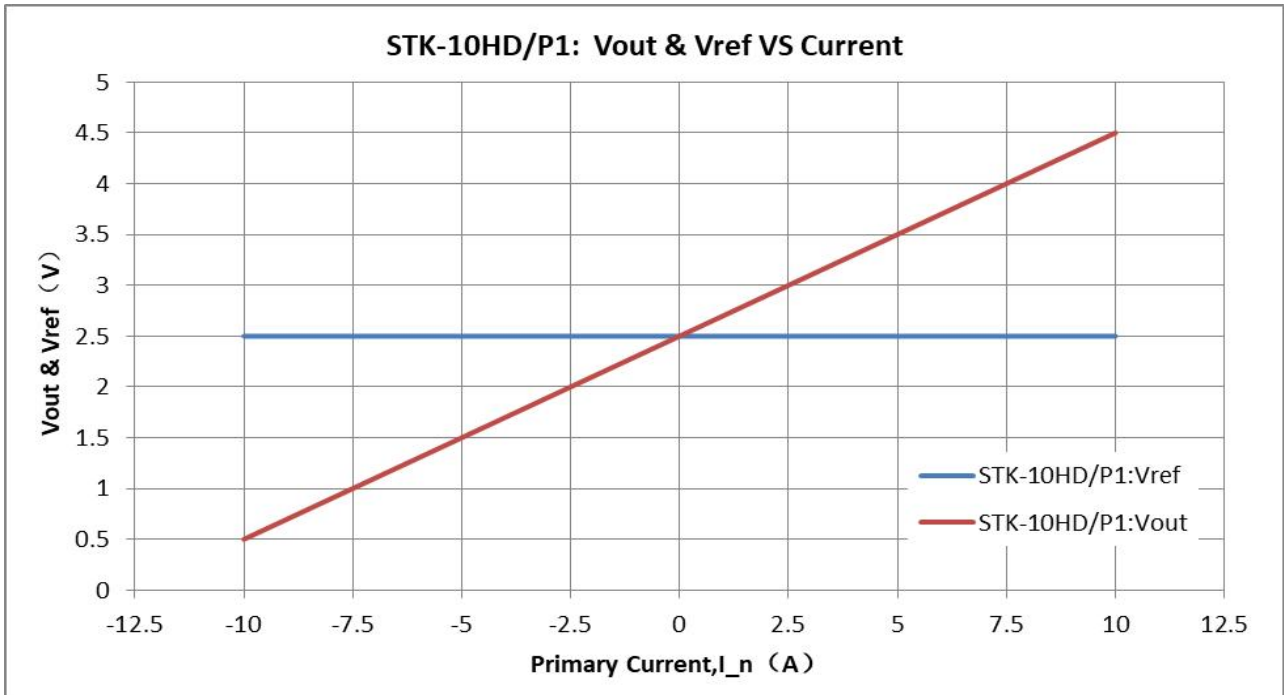
The dependence of Vout of STK-10HD/P1 on the primary current.
