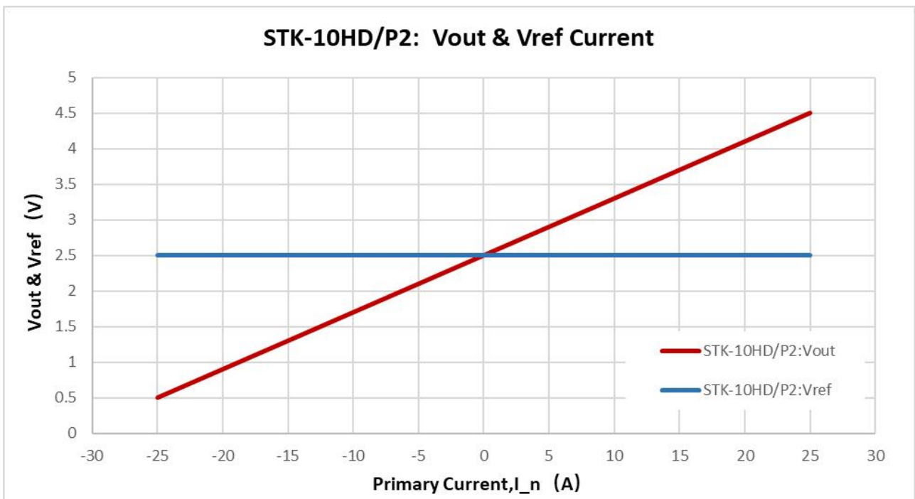
The dependence of Vout of STK-10HD/P2 on the primary current.
